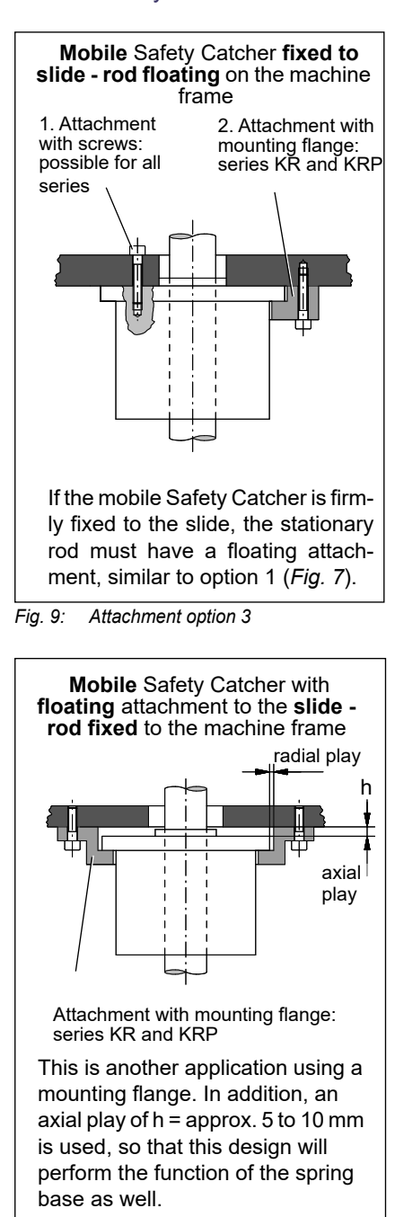
Fig. 10: Attachment option 4
