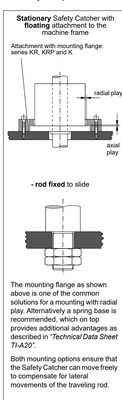
Fig. 8: Attachment option 2
