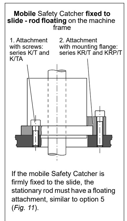
Fig. 13: Attachment option 3
