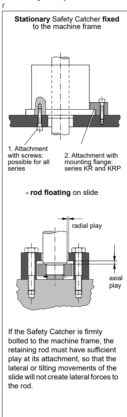
Fig. 7: Attachment option 1
